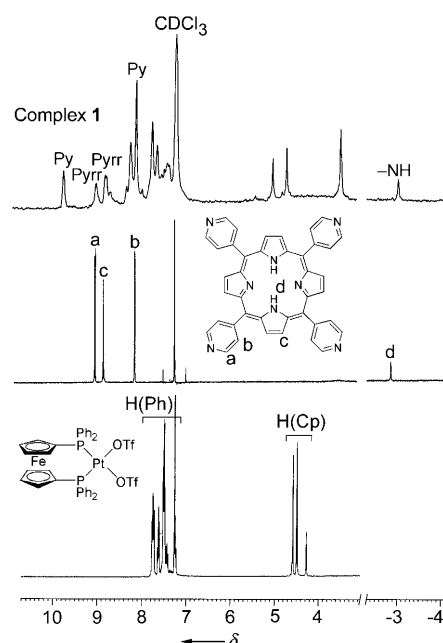
Figure 1. ^1\text{H} NMR spectra of the complex 1 and linkers L and M in \text{CDCl}_3 .
