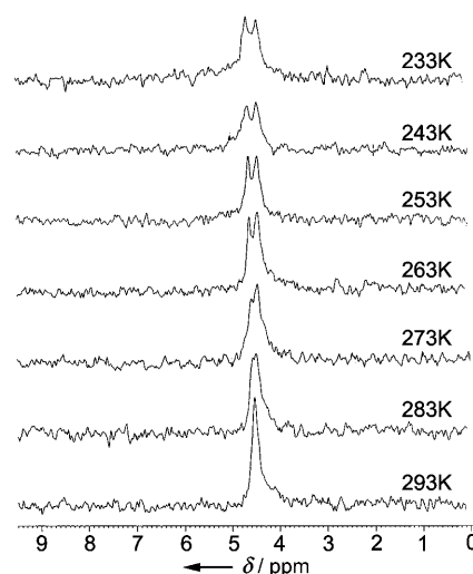
Figure 4. Variable-temperature ^{31}\text{P} NMR spectra of the complex 1 in \text{CD}_3\text{OD} .
